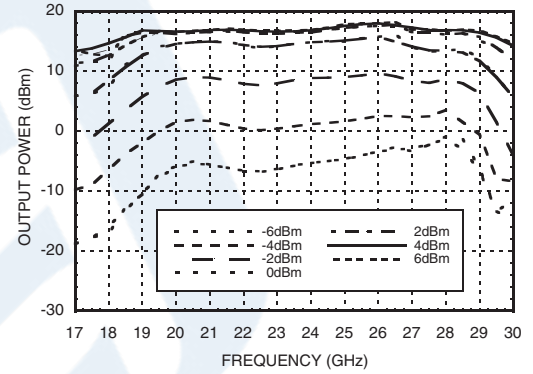
Output Power vs. Drive Level
